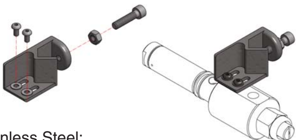
Kit 04 Direct Mount V-Block Bracket
