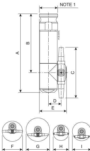
Figure 2. 4-nozzle
