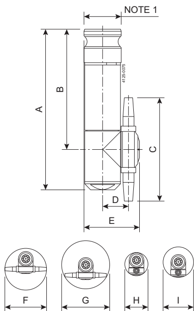
Figure 1. 2-nozzle
