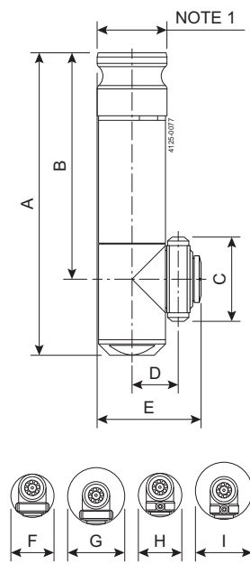
Figure 3. Low-profile
